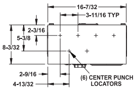
225 Amp Typical Top View for NEMA 3R
