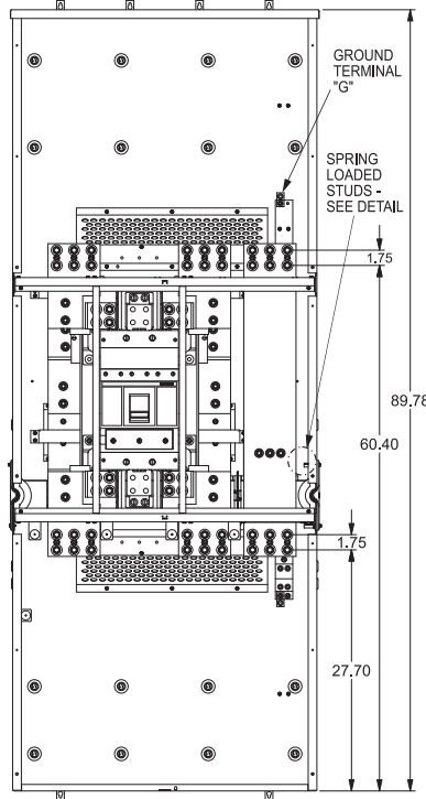
VIEW SHOWN WITHOUT COVERS
