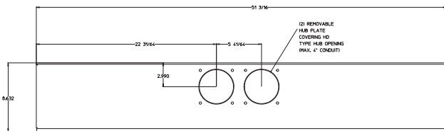
Top view for WEP6512 and WEP6612
