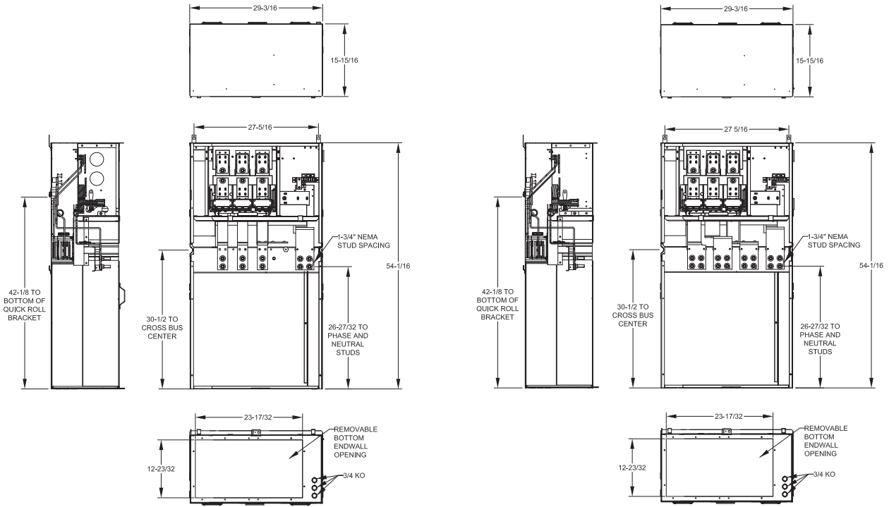
ES-1 WES1400BU WES3400BU
