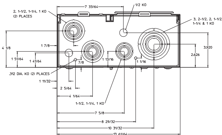
Bottom view for WP2211 and WEP2211
